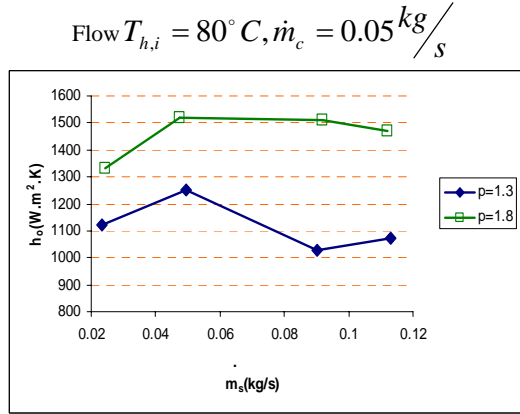
Fig. 16. Shell side heat transfer coefficient in relation to the crust
