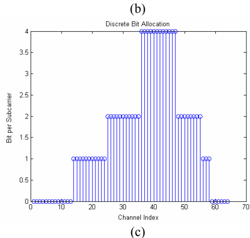
Fig. 2 Example optimal Bit and Energy Allocation
