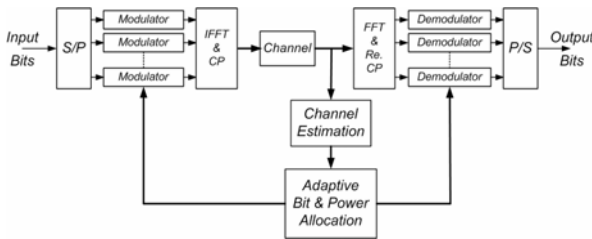
Fig. 1 OFDM System block Diagram
