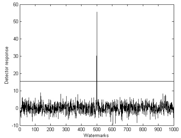
Fig. 8 Ellinas et al detector response for "Lena"
