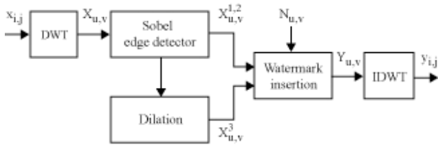
Fig. 1 Block diagram of the watermark insertion process
