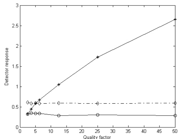
Fig. 9 Detector response versus JPEG quality factor
