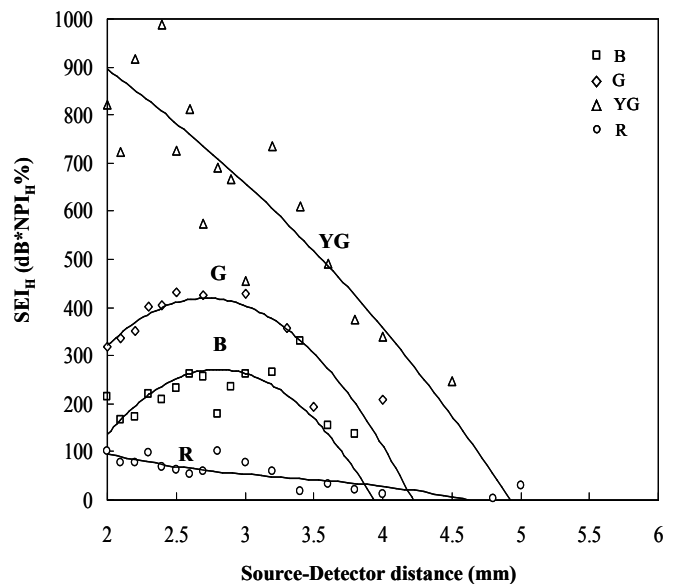
Fig. 7 The signal-effect-index ( SEI_H ) at different emitter-detector distance
