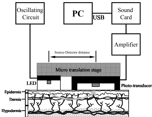
Fig. 1 Measurement setup of reflectance photoplethysmograph
