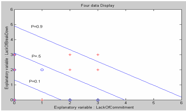
Fig. 2 Four data display: two numerical predictors "lack of break down", "lack of commitment" and the binary outcome. (+) denotes a response with y_i=1 , (o) denotes a response with y_i=0 . The contour lines are displayed as a function of the probability of occurrence.
