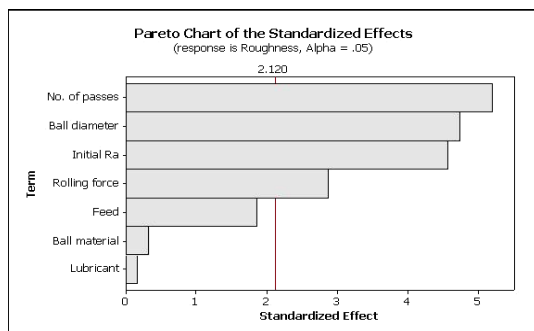
Fig. 7 Pareto chart for surface roughness
