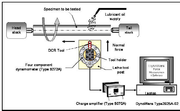
Fig. 3 Deep cold rolling setup
