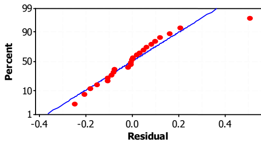
Fig. 5 Normal probability plot for surface roughness
