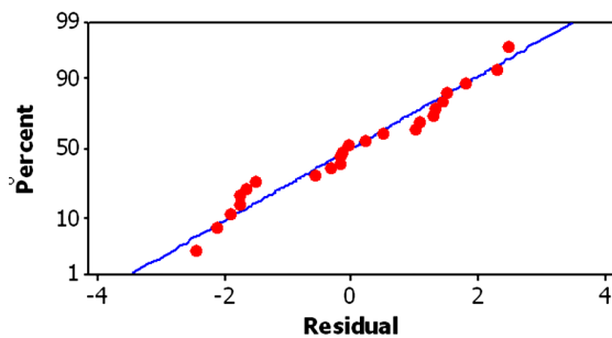
Fig. 6 Normal probability plot for surface hardness
