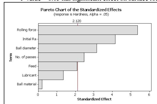
Fig. 8 Pareto chart for surface hardness
