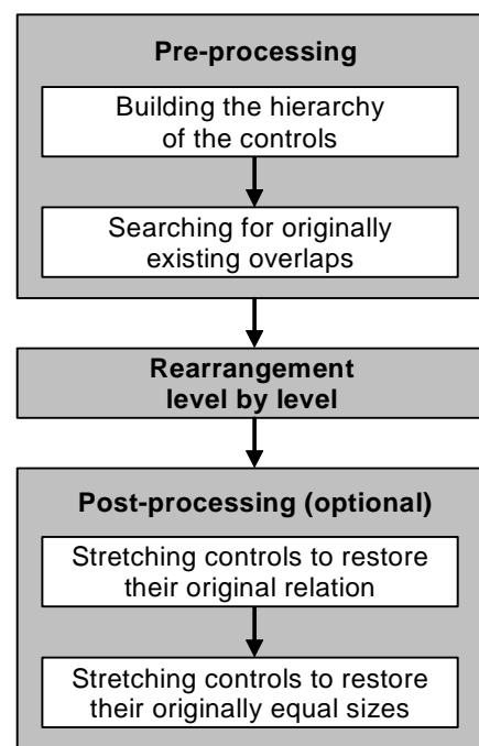
Fig. 2 Phases of the rearrangement algorithm
