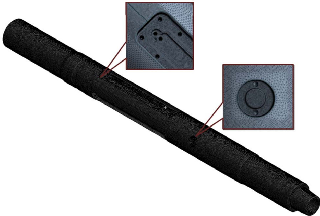
Fig. 2 Mesh Details
