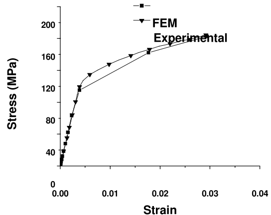
Fig. 11 Comparison of experimental and FE simulation stress-strain curves for buffalo femoral cortical bone
