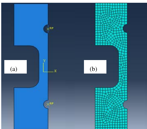
Fig. 7 Diagram showing the finite element model of sub-size specimen (a) two dimensional half model of sub-size specimen (b) model of sub-size specimen along with mesh.
