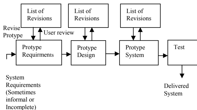
Fig. 2 Iterative Method Outline
