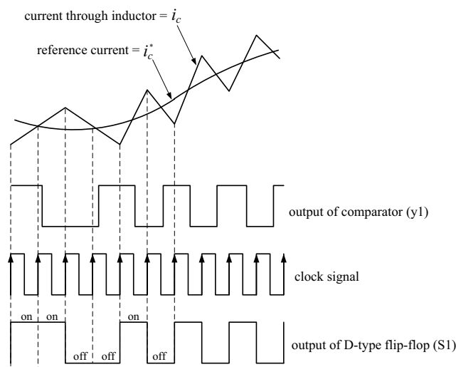
Fig. 7 The basic concept of the delta modulation current control
