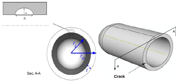
Fig.2 Schematic of a pressure vessel with an elliptical crack
