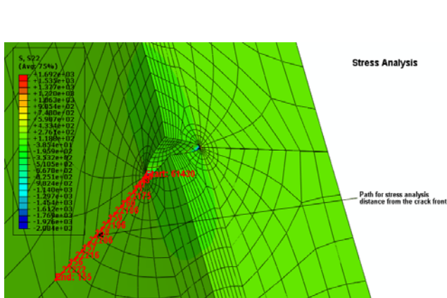
Fig.11 contour of stress near the crack front for mode I Stress
