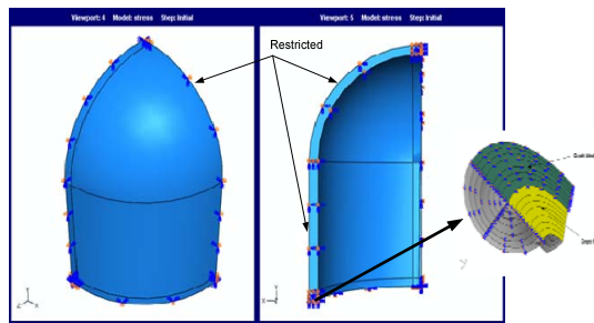
Fig.8 Schematic of 1/8 pressure vessel with boundary conditions
