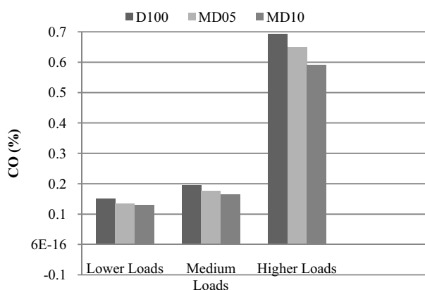
Fig. 9 Emission of CO at various loads
