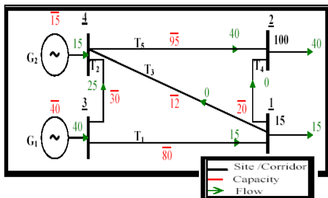
Fig. 1 A Sample power system
