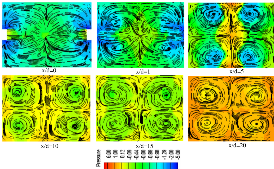
Fig. 7 cross-stream pressures streamline plots at six downstream locations, showing the initiation and formation of streamwise vortices
