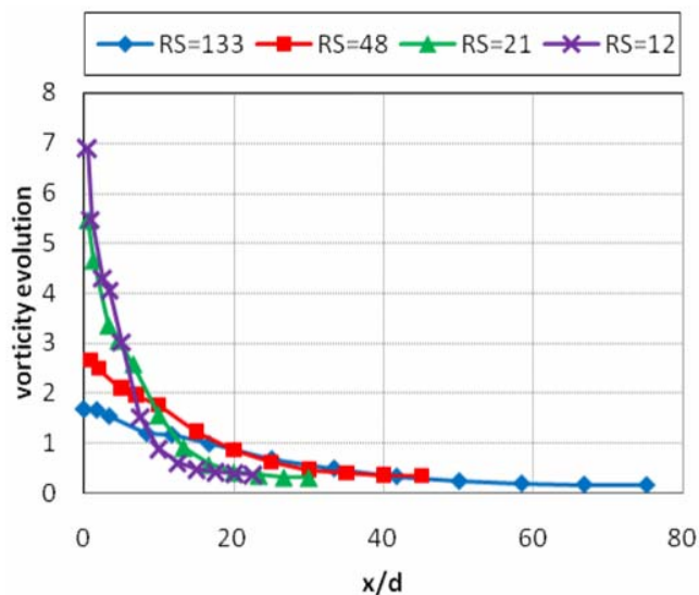
Fig. 11 Total vorticity evolution
