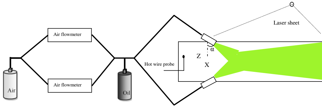
Fig. 1 Sketch of the experimental set-up
