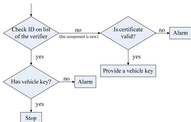
Fig. 2 Security check process example
