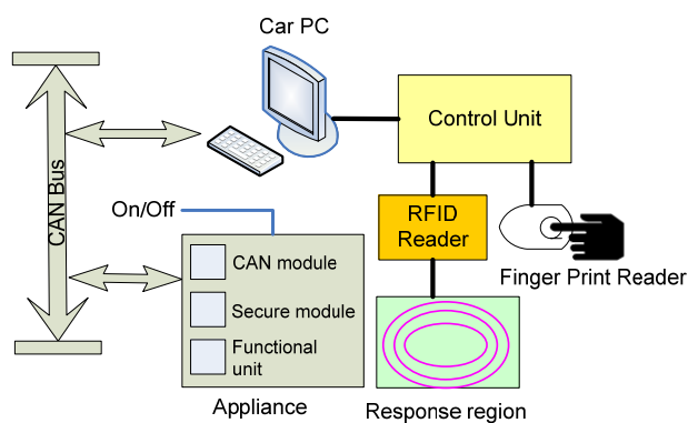
Fig. 3 System Architecture
