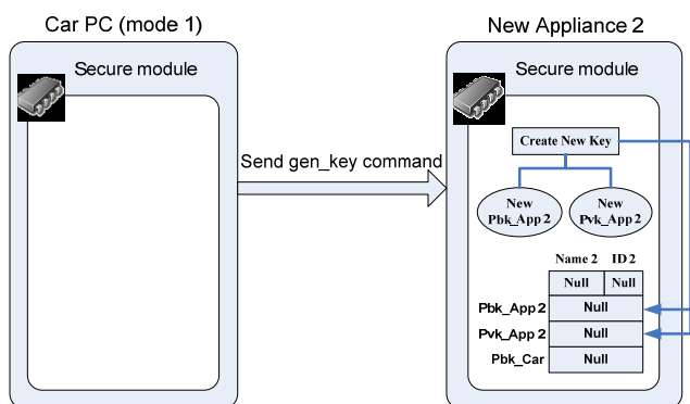
Fig. 7 Mode-1 for installing the new appliance
