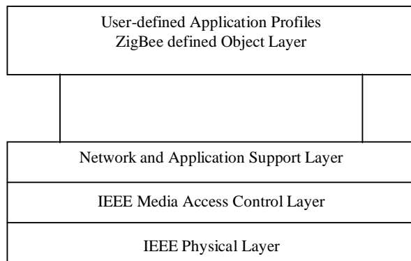
Fig. 3 IEEE 802.15.4 / ZigBee Stack Architecture
