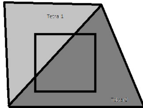
Fig. 5. 2-D example of voxel generation : m(V_j) = m(I_1^j) + m(I_2^j)
