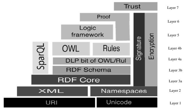
Fig. 4 Semantic Web Layered Architecture V3 [6]
