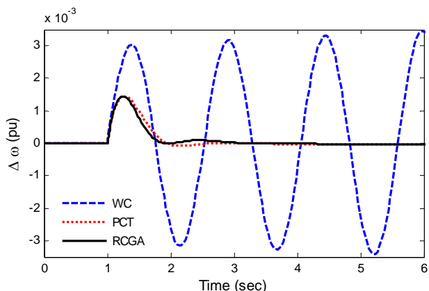
Fig. 9. Speed deviation response for Case-III
