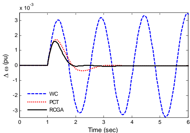
Fig. 11. Speed deviation response for Case-IV
