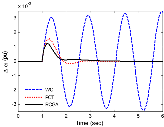
Fig. 5. Speed deviation response for Case-I
