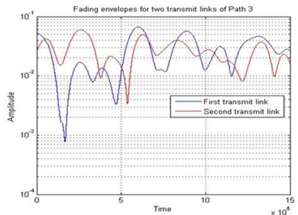
Fig. 10: Fading envelopes for two transmitted links of path 3 in SUI2
