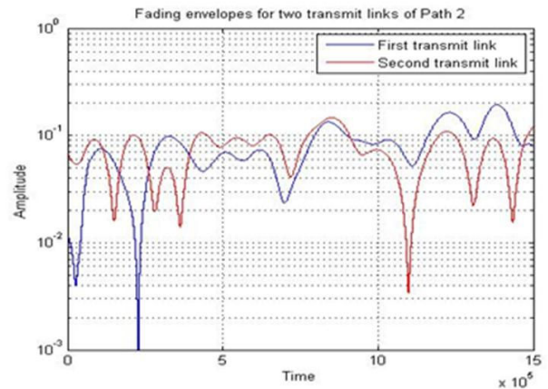
Fig. 9: Fading envelopes for two transmitted links of path 2 in SUI2
