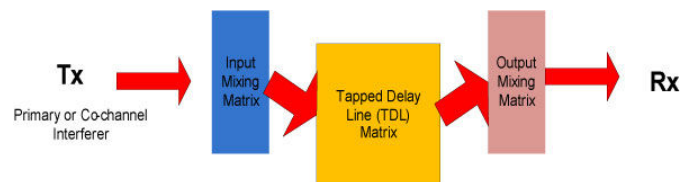
Fig. 1: Generic Structure for SUI Model
