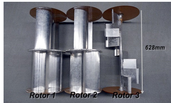
Fig. 4 Fabricated Rotor 1, 2 and 3
