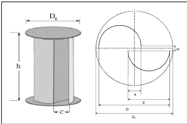
Fig. 1 Schematic Drawing of rotor 1
