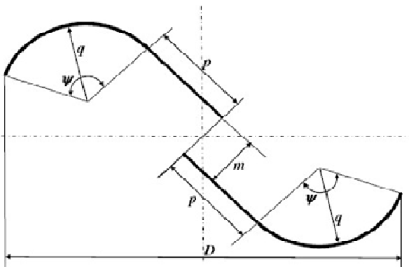
Fig. 2 Schematic drawing of rotor 2
