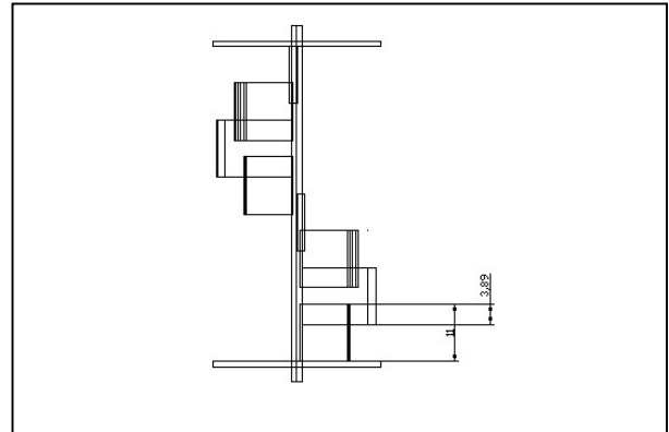
Fig. 3 Schematic Drawing of rotor 3
