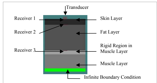
Fig. 1 Two-Dimensional FD model and its elements; Model type (normal or rigid model) was determined with the material properties used in the rigid region in the muscle layer
