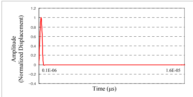
Fig. 2 Source signal (5MHz frequency with amplitude of 1) applied to the FD models during 0.1μs
