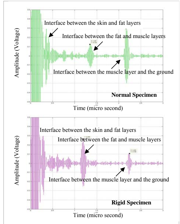
Fig. 7 Representative ultrasonic responses for the normal and rigid specimens determined from the actual ultrasound system
