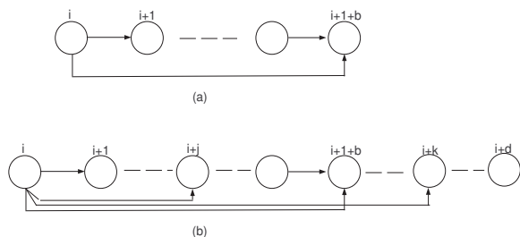
Fig. 3. AUTHENTICAST hash-chaining with k = 4 .
