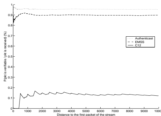
Fig. 5. Average verification probability
