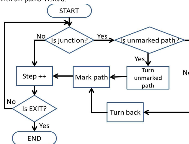
Fig. 2 Tremaux's algorithm [4]
