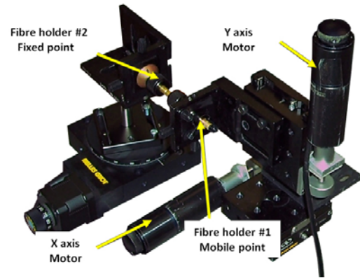
Fig. 1. Positioning Stage
