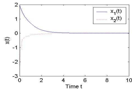
Fig.1 Responses of system states
