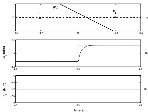
Fig. 12. Stable velocity transient crossing ( D_1 ), from P_1 to P_2 , in regenerating mode (quadrant 4) (a), from \omega_o = 14.7 rad/s to \omega_o = 15.3 rad/s (b), nominal torque ( T_{Lo} = -7N.m ) (c), K_i = 3000 , K_p = 300 .
