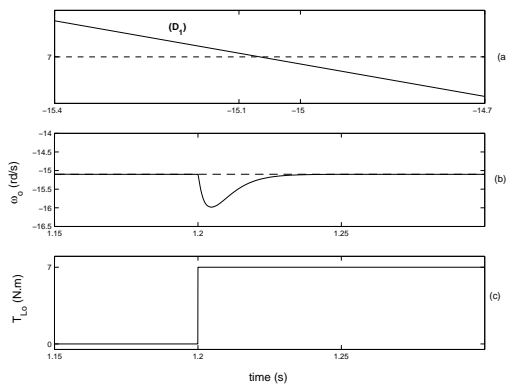
Fig. 11. Velocity transient in the vicinity of ( D_1 ) in regenerating mode (quadrant 2) (a), from T_{Lo} = 0 N.m to T_{Lo} = 7 N.m (c), low velocity ( \omega_o = 15, 1rd/s ) (b), K_i = 3000 , K_p = 300 .
