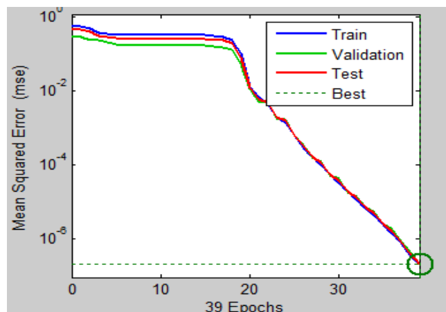
Fig. 9 Data validation with best performance at 39 epoch
