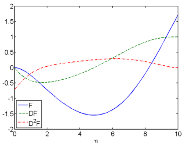
Fig. 4. Similarity solutions of reversed stagnation-point flow
