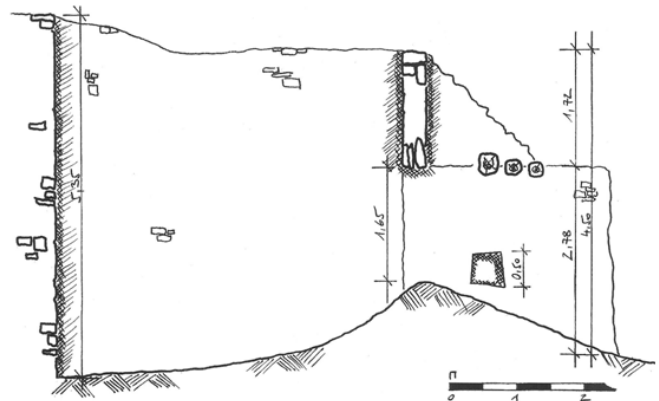
Fig. 5 Section of Lime Kiln 1
