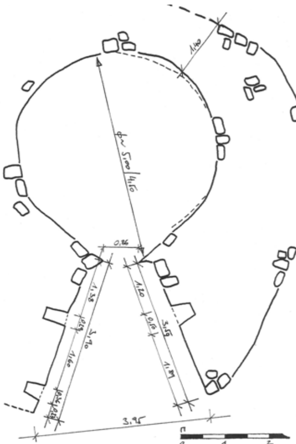
Fig. 4 Ground plan of Lime Kiln 1
