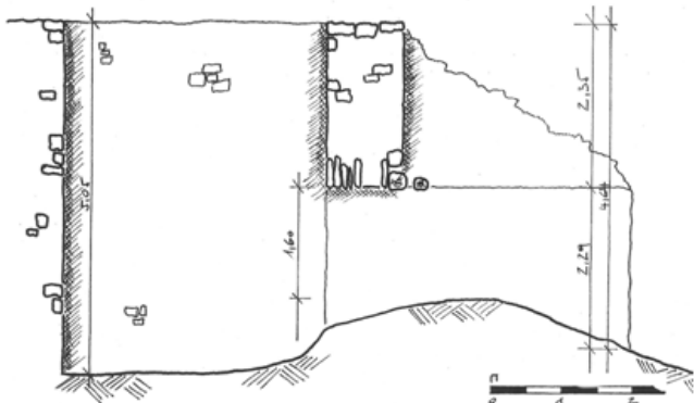
Fig. 8 Section of Lime Kiln 2
