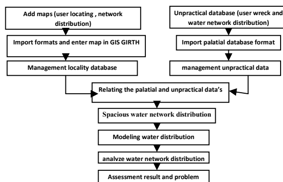
Fig. 1 water distribution network modeling process
