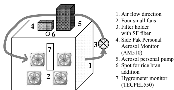
Fig. 1 Schematic diagram of the reactor
