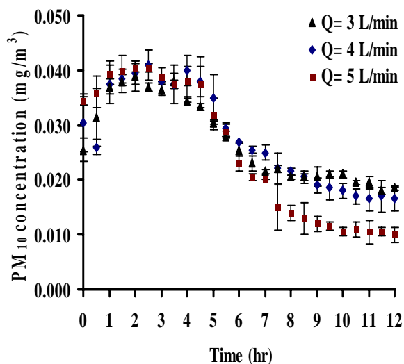
Fig. 3 PM 10 concentration before and after treatment
