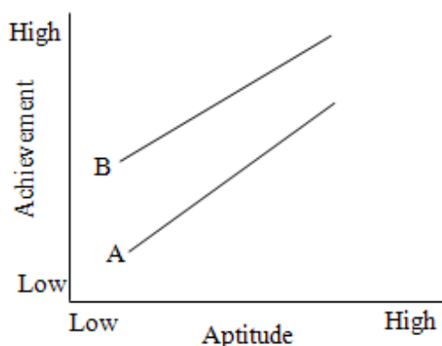
Fig. 3 Ordinal Interaction
