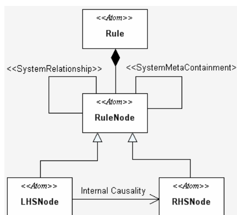
Fig. 3 The metamodel of the VMTS Rule Editor
