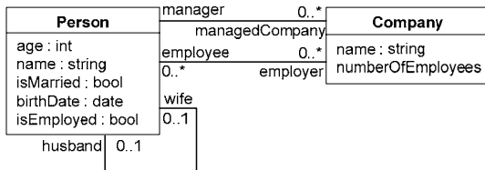
(a) Metamodel:
