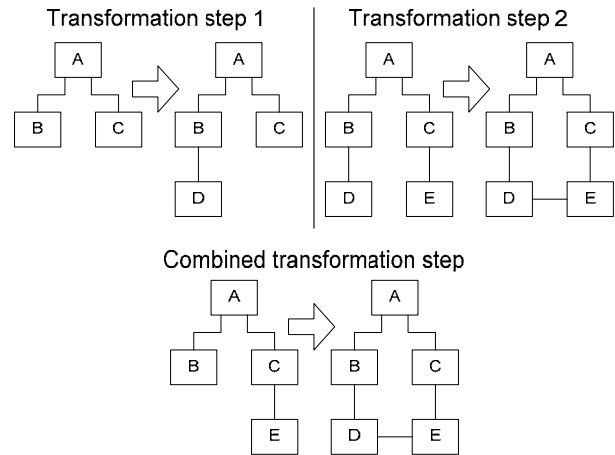
Fig. 7 An example for transformation step combination
