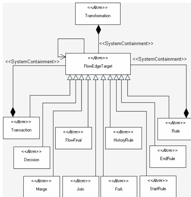
Fig. 2 The metamodel of the VMTS Visual Control Flow Language
