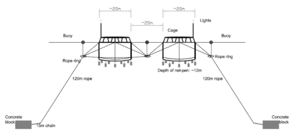
Fig. 6 Side-view of aquaculture cages
