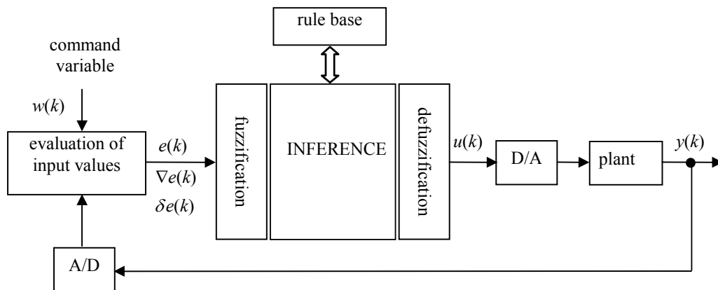
Fig. 4 A block diagram of fuzzy control
