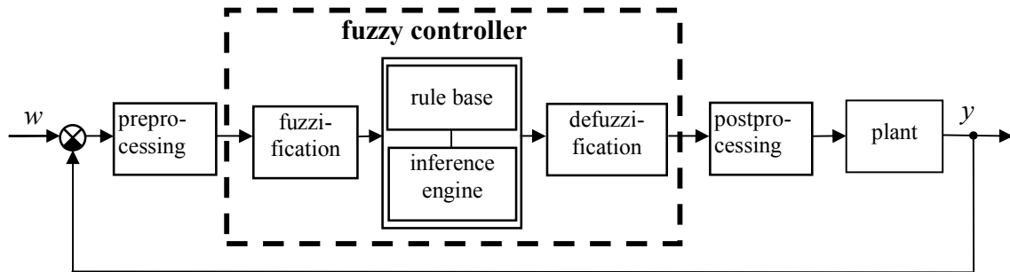
Fig. 2 Feedback control with a fuzzy controller
