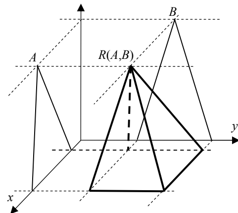
Fig. 1 Mamdani implication
