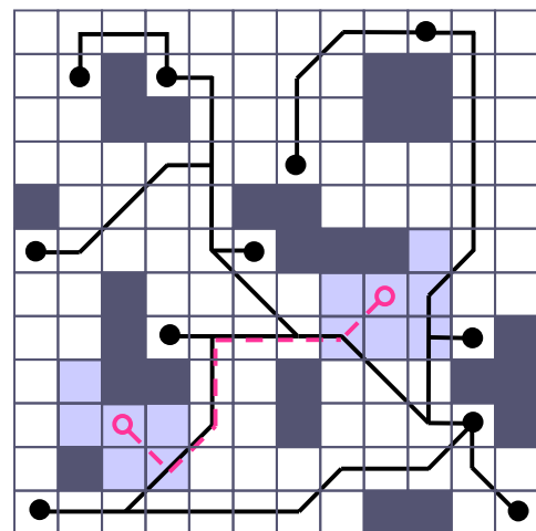
Fig. 9 "Neighbour-intersection" strategy
