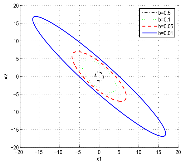
Fig. 3. The size of attraction region according to increasing b
