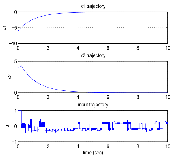
Fig. 2. The states and input trajectories
