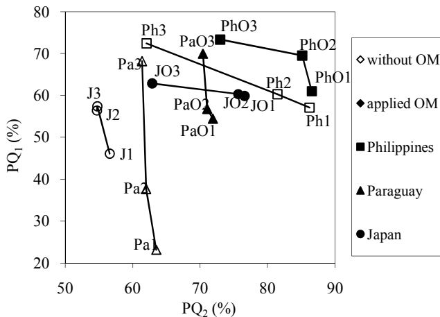
Fig. 3 Relationship of percent of humic acid in extracted humus by \text{NaOH} ( \text{PQ}_1 ) and \text{Na}_4\text{P}_2\text{O}_7 ( \text{PQ}_2 ) in soils studying after 6 months incubation
