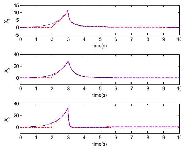
Fig. 1 Actual states (line), state estimations (dashed)
