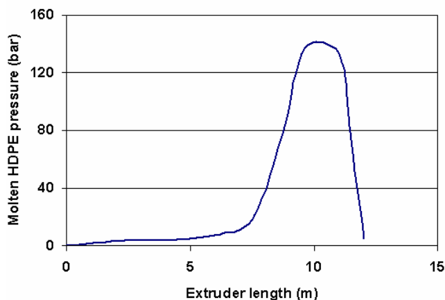
Fig. 2 Pressure profile in twin-screw extruders' length
