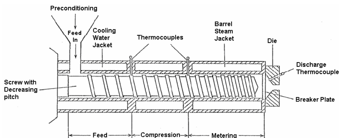
Fig. 1 Single-screw extruder
