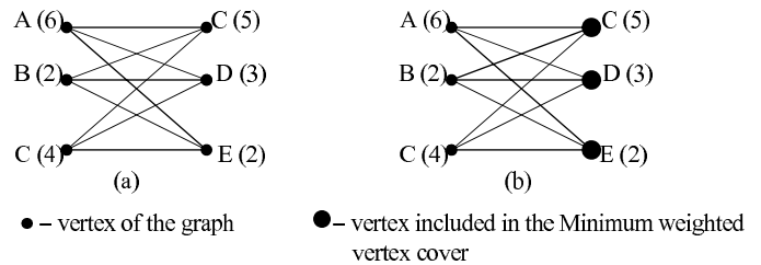
Fig. 1. (a) Graph G(V,E) (b) G(V,E) with MWVC
