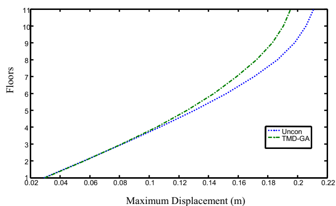
Fig. 14. Maximum displacement of floors under Tabas 1999 earthquake.
