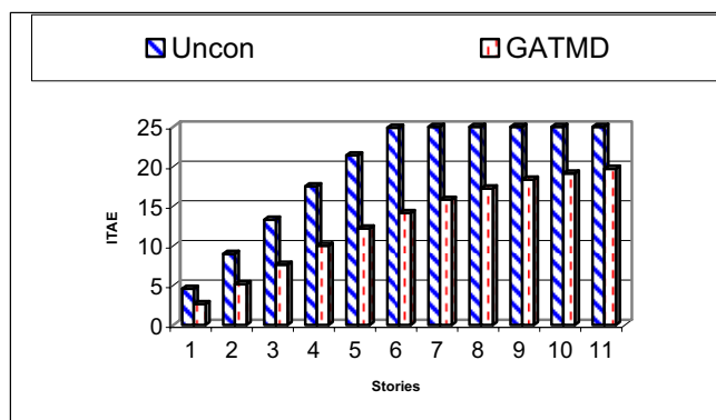
Fig. 15. ITAE performance index value for all floors under Tabas earthquake.
