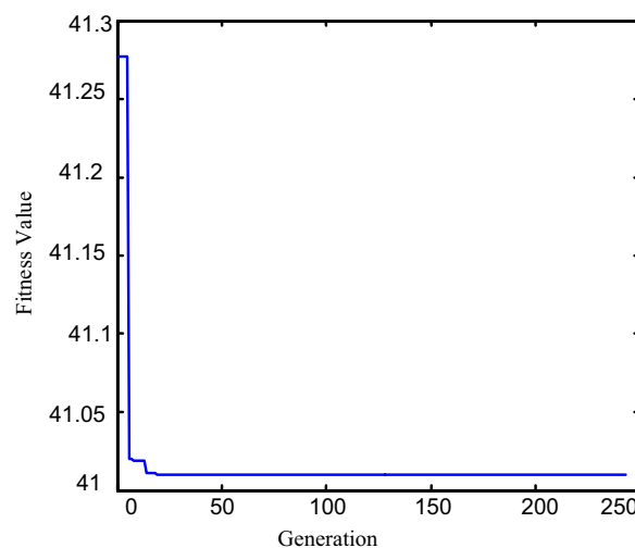
Fig. 6. Minimum fitness convergence by GA.
