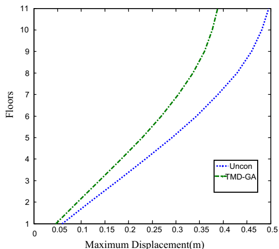
Fig.11. Maximum displacement of floors under Kobe 1995 earthquake.
