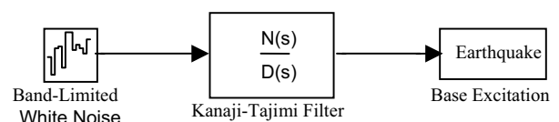
Fig. 5. Base excitation used for tuning of the TMD Parameters.
