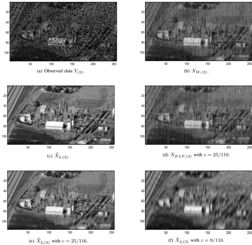
Fig. 2. Illustration to signal X_{(3)} estimation by different filters. Here, X_{W,(3)} is the estimate by the Wiener filter, \tilde{X}_{2,(3)} is the estimate that follows from (5) with p = 3 , X_{KLF,(3)} is the estimate by KLF with c = 25/116 , \hat{X}_{2,(3)} is the estimate that follows from (6)-(7) with c = 25/116 , and \bar{X}_{2,(3)} is the estimate that follows from (6)-(7) with c = 9/116 .
