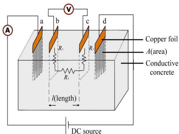
Fig. 1. Structure of the four-electrode method.
