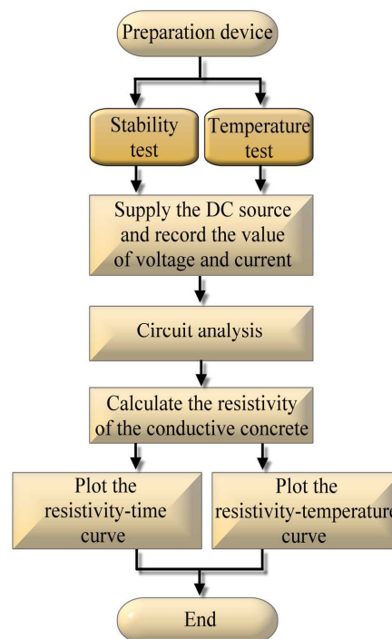
Fig. 3. Flowchart of the resistivity measurement.
