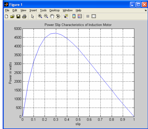
Fig. 3 Power slip characteristic of induction motor
