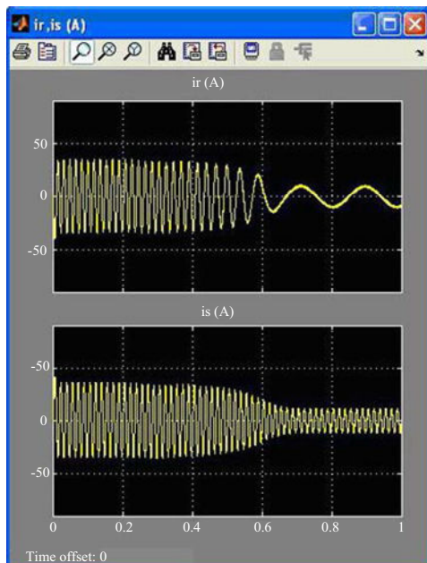
Fig. 9 Stator and Rotor current of three-phase induction motor
