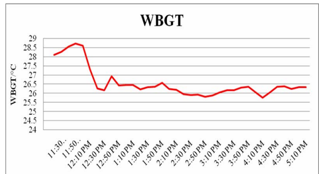
Fig. 5 WBGT measured at the body assembly station
