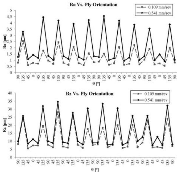
Fig. 10 Comparison of roughness parameters R_a and R_z for 2 feed rates at 800 m/min
