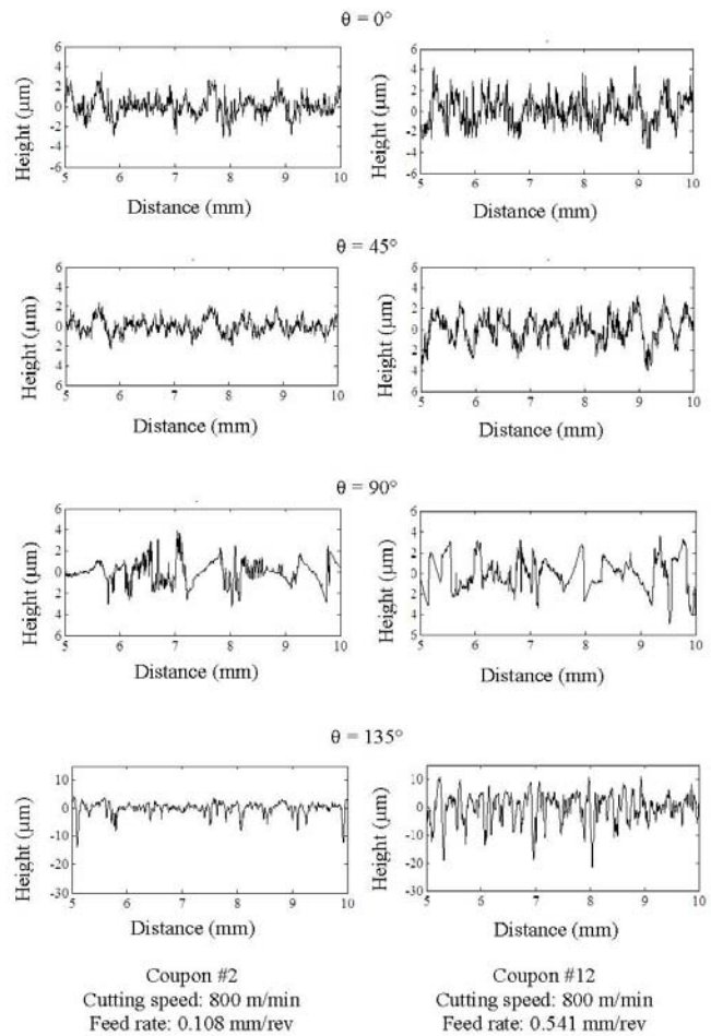
Fig. 9 Effect of feed rate on roughness profiles
