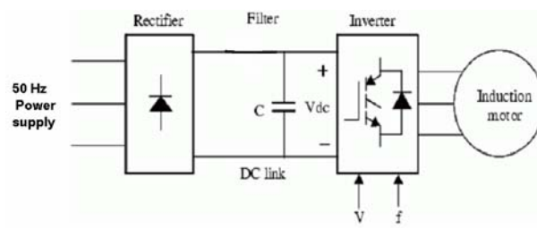
Fig. 2 VSI fed Induction motor
