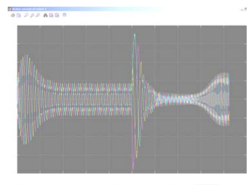
Fig. 8 (a) Waveform for Stator current of motor 2 for change in ref speed
