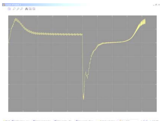
Fig. 8 (c) Waveform for torque of motor 2 for change in ref. speed
