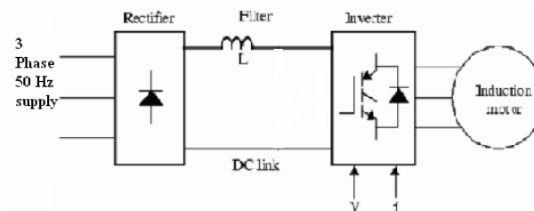
Fig. 3 CSI fed Induction motor
